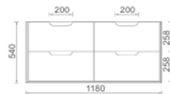
SYWH04-1200D-NEW Size:1180*455*540mm
