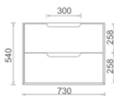
SYWH04-750-NEW Size:730*455*540mm
