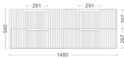
WH86-1500D-NEW Size: 1480x455x540mm
