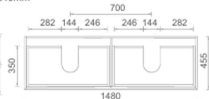
SYWH04-1500D-NEW Size:1480*455*540mm
