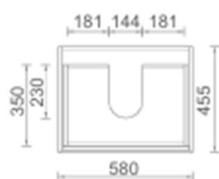
SYWH04-600-NEW Size:580*455*540mm
