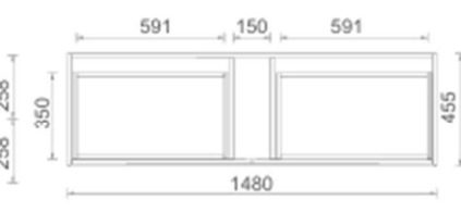
SYWH04-600S-NEW Size:580*455*540mm
