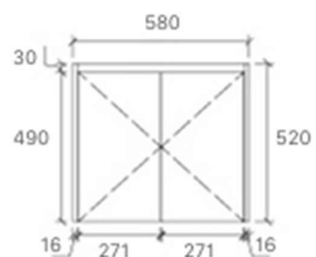
SYWH05-600 Size: 580x455x520mm
