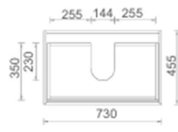
SYWH04-750-NEW Size:730*455*540mm
