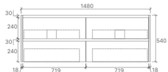
YOKO-1500D Size: 1480x455x540mm
